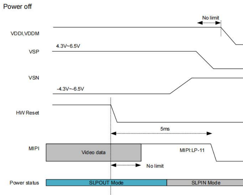
Figure 4.3: Power-Off sequence
